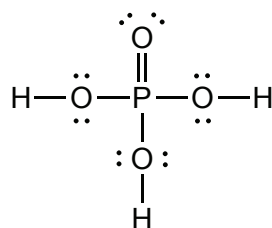
Lewis formula 2
